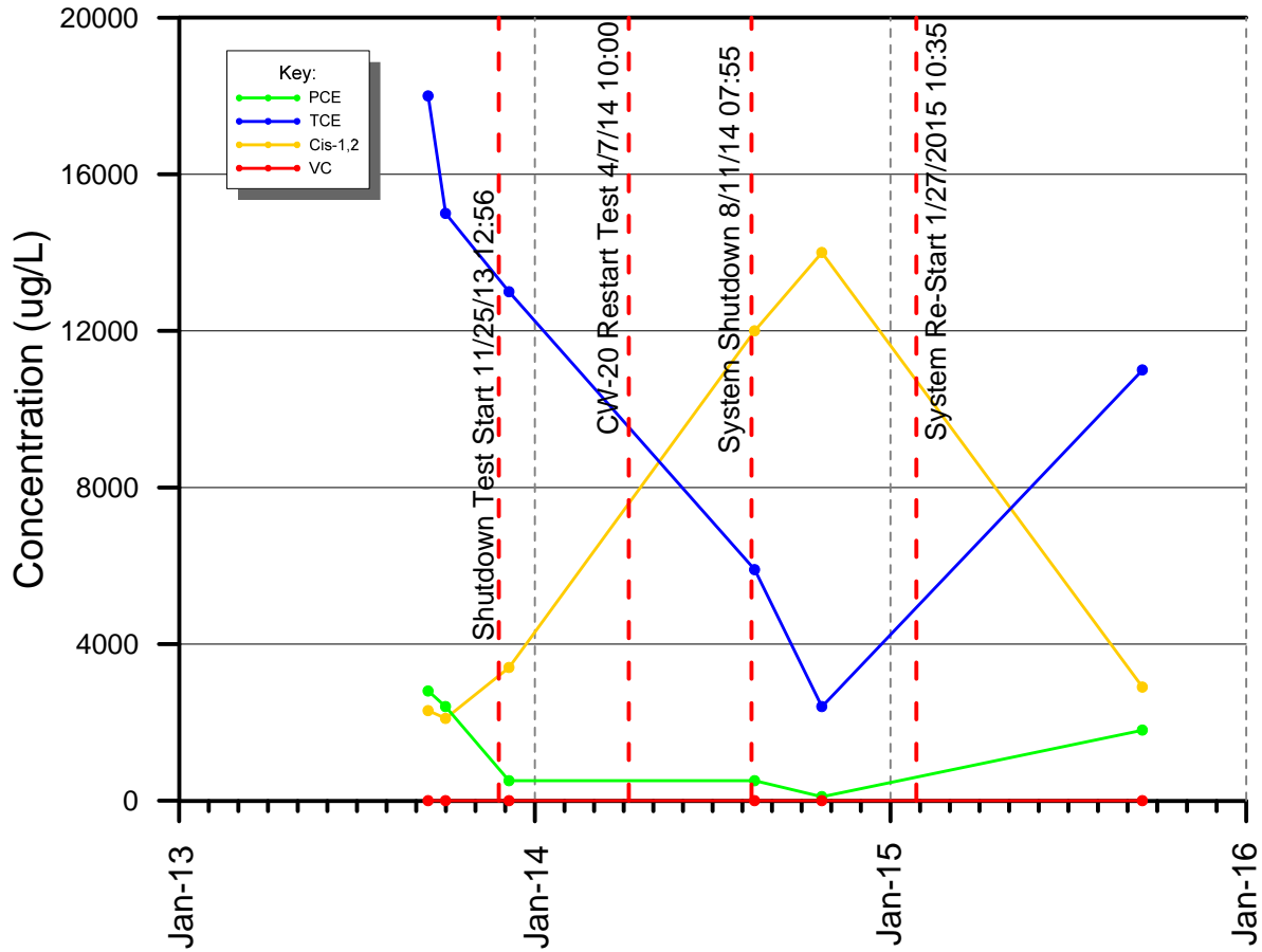
Figure 2.2-4 MW-136A(434-434.5) Chemistry Graphs - Ethenes
